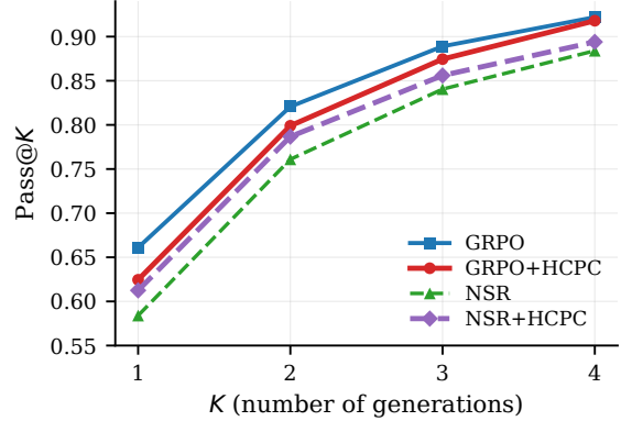
Figure 2: Pass@ K on ChartFC (OOD, n=500 ). Plain NSR (green) sits below all other configurations at every K ; adding HCPC (purple) closes most of the gap to GRPO. BASE was not evaluated on ChartFC.
